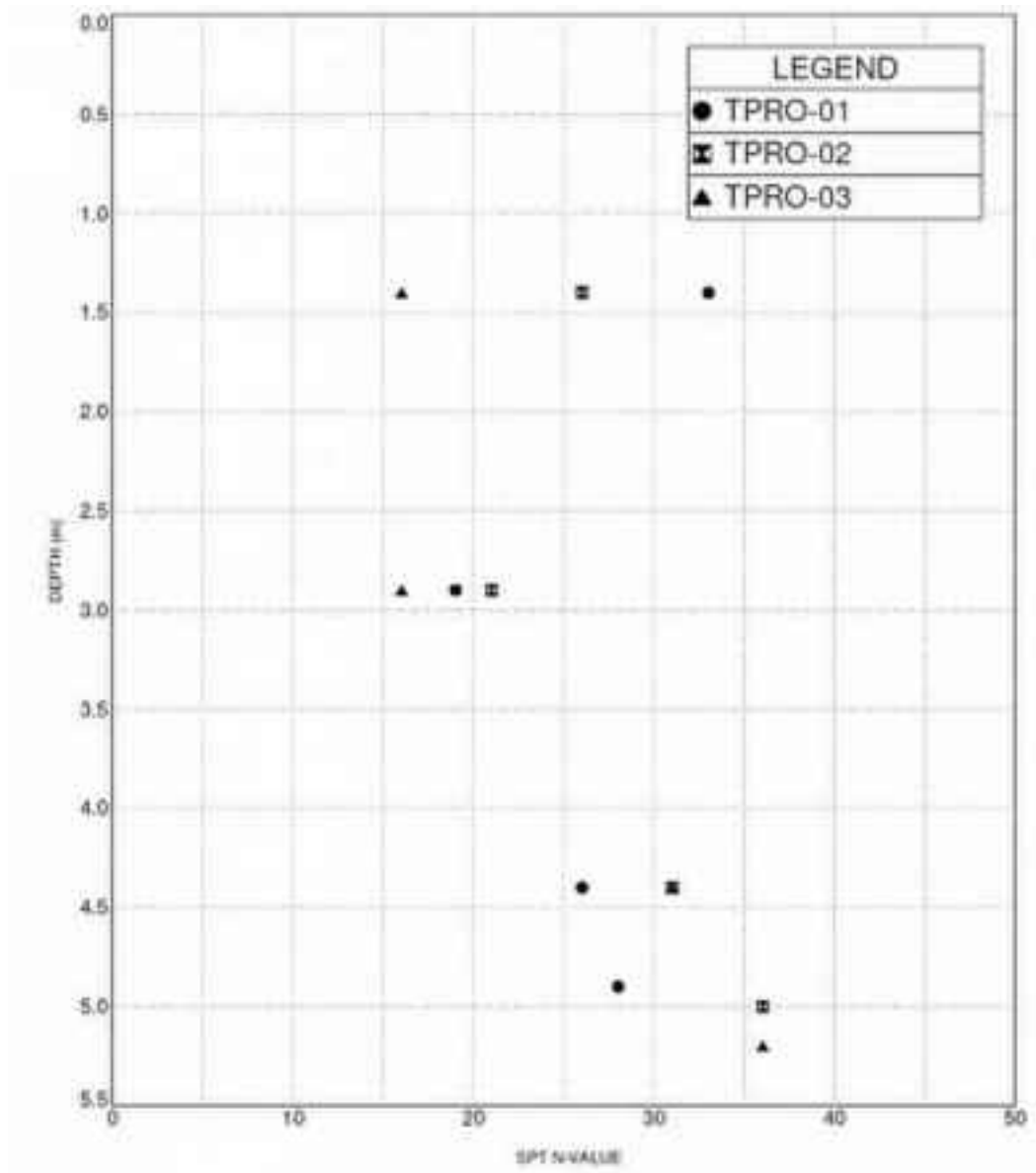
Figure 6 – SPT Vs Depth plot for Open-holes TPRO-01, 02 & 03
